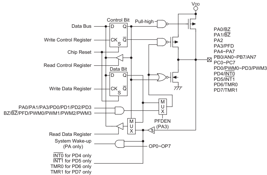
Input/Output Ports
