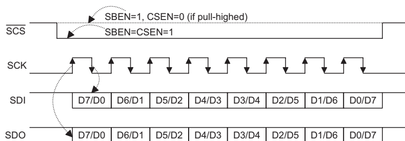
SIO Timing (SIOCLK Configuration is Rising Edge)
