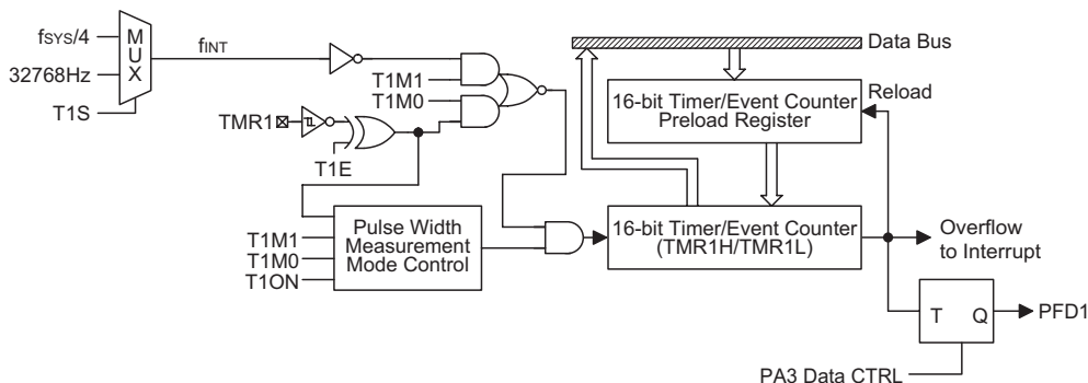
Timer/Event Counter 1
