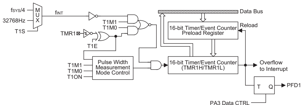
Timer/Event Counter 1
