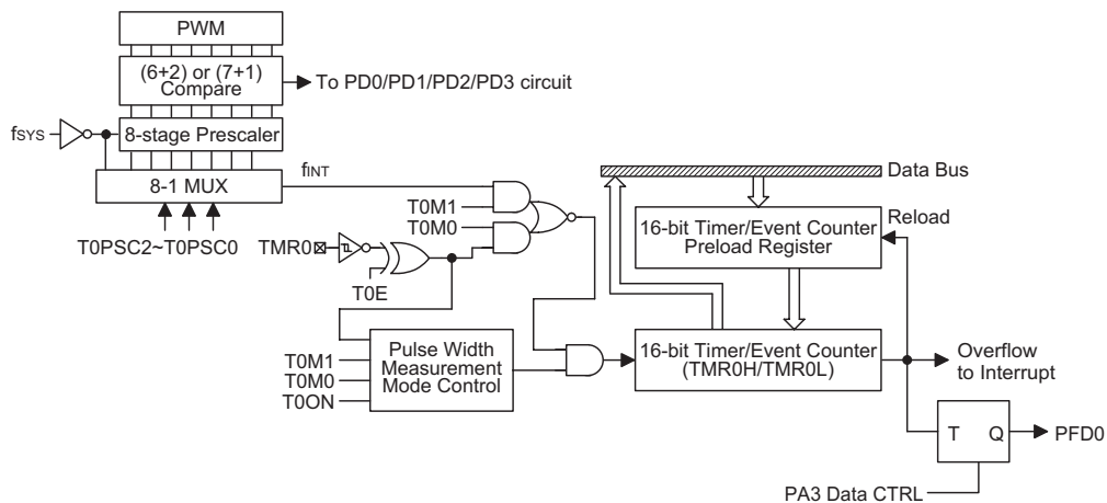
Timer/Event Counter 0
