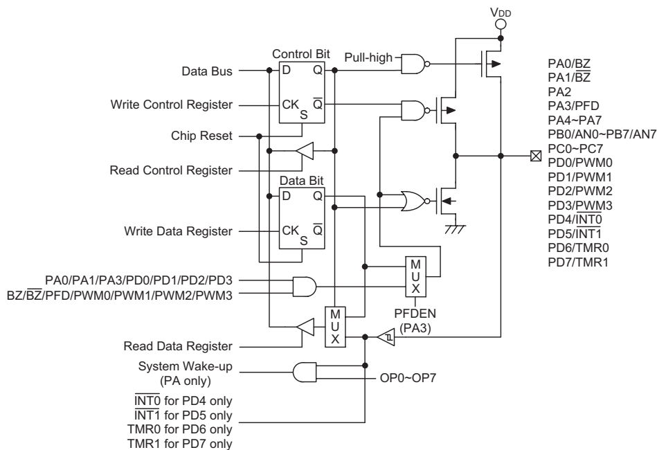
Input/Output Ports
