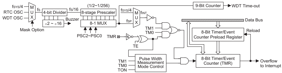
Timer/Event Counter and WDT
