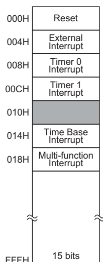
Program Memory Structure
