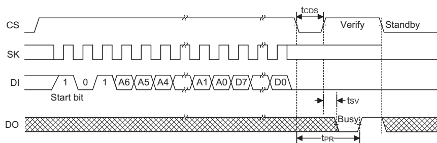
WRITE Timing
