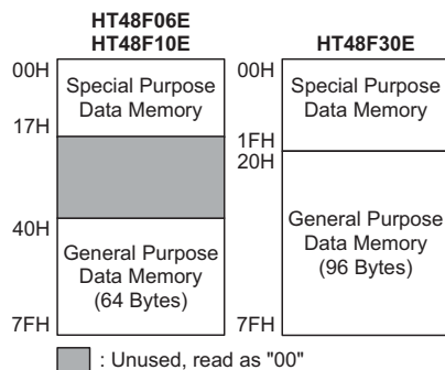
Bank 0 RAM Data Memory Structure
