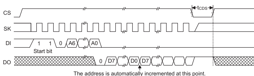
READ Timing
