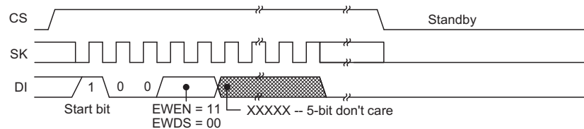
EWEN/EWDS Timing
