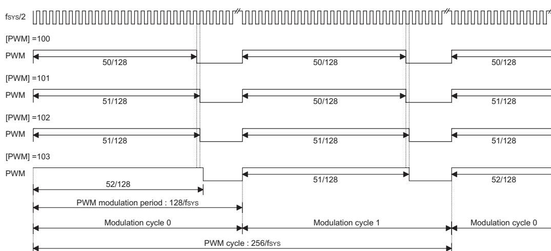
(7+1) PWM Mode
