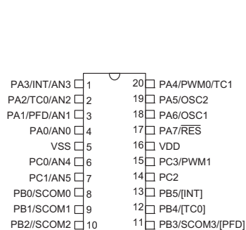
HT46R066 20 DIP-A/SOP-A/SSOP-A
