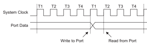
Read/Write Timing
