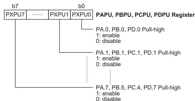
Pull-High Resistor Register – PAPU, PBPu, PCPU, PDPu
