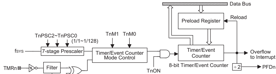
8-bit Timer/Event Counter Structure (n=0, 1)
