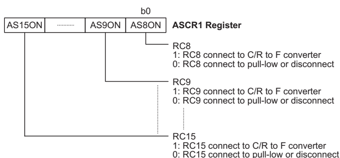
ASCR1 Register
