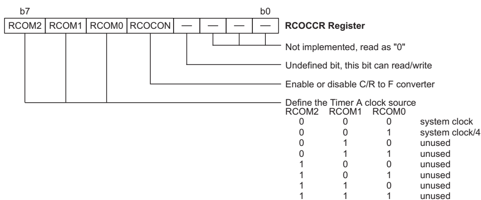
RCOCCR Register
