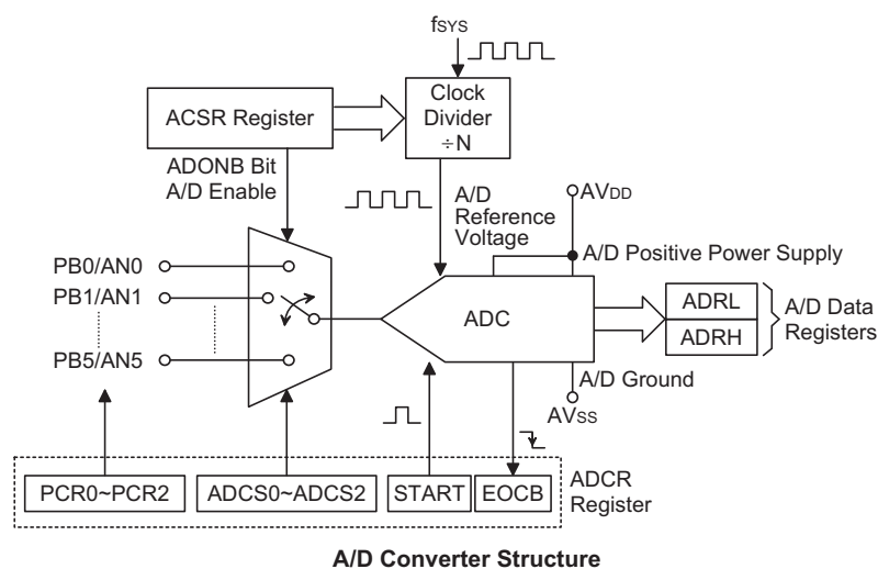
A/D Converter Structure
