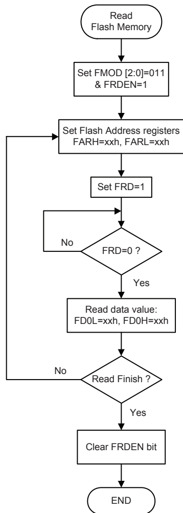
Read Flash Memory Procedure
