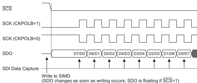
SPI Slave Mode Timing — CKEG=0
