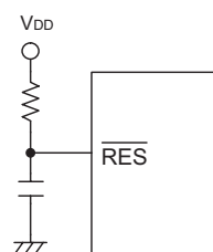
Reset Circuit
