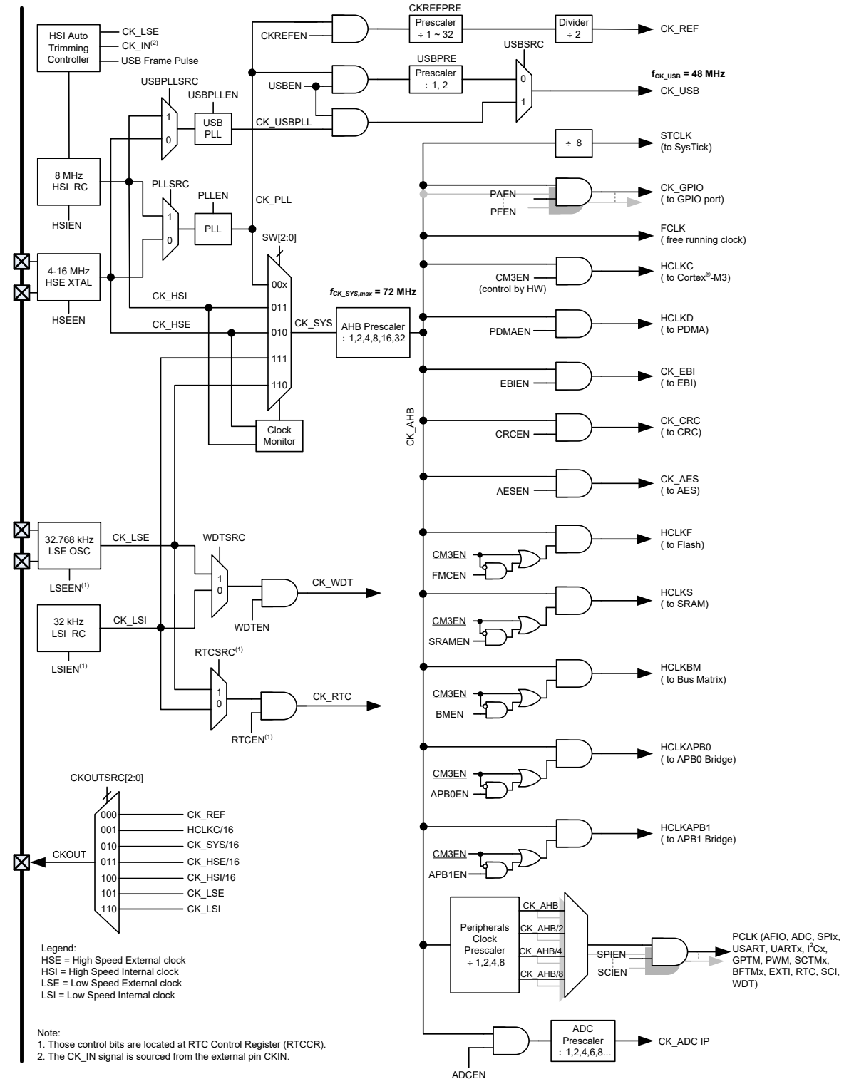
Figure 3. Clock Structure
