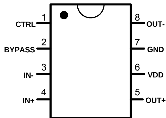
8-pin SOP Top View
