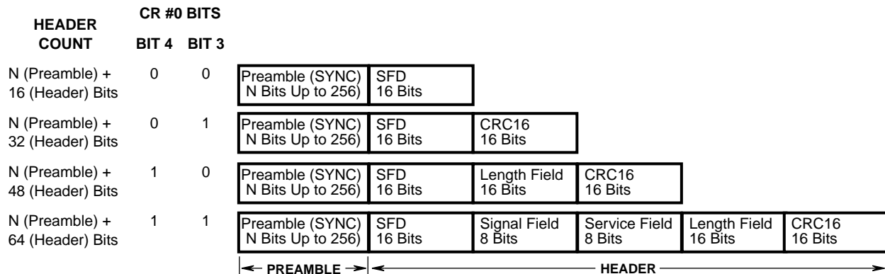
FIGURE 10. PREAMBLE/HEADAR MODES
