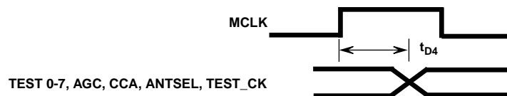
FIGURE 26. MISCELLANEOUS SIGNAL TIMING
