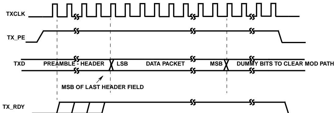
FIGURE 6. TX PORT TIMING (INTERNAL PREAMBLE)
