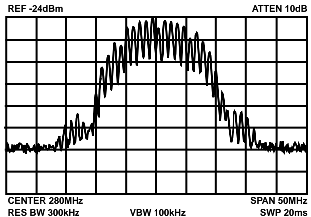
FIGURE 11. UNSCRAMBLLED DBPSK DATA OF ALTERNATE 1's/0's SPREAD WITH AN 11-BIT SEQUENCE
