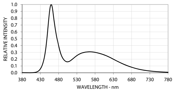
Figure 4. Spectrum
