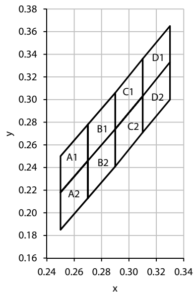
Figure 1. Chromaticity diagram
