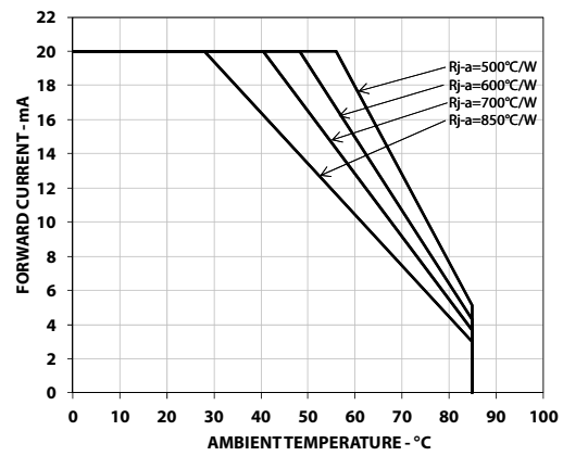
Figure 8. Derating curve
