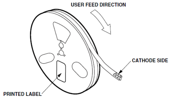
Figure 10. Reel orientation
