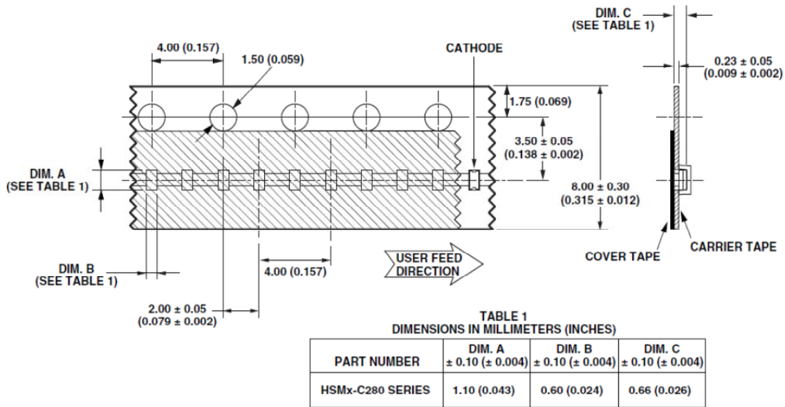
Figure 12. Carrier tape dimensions
