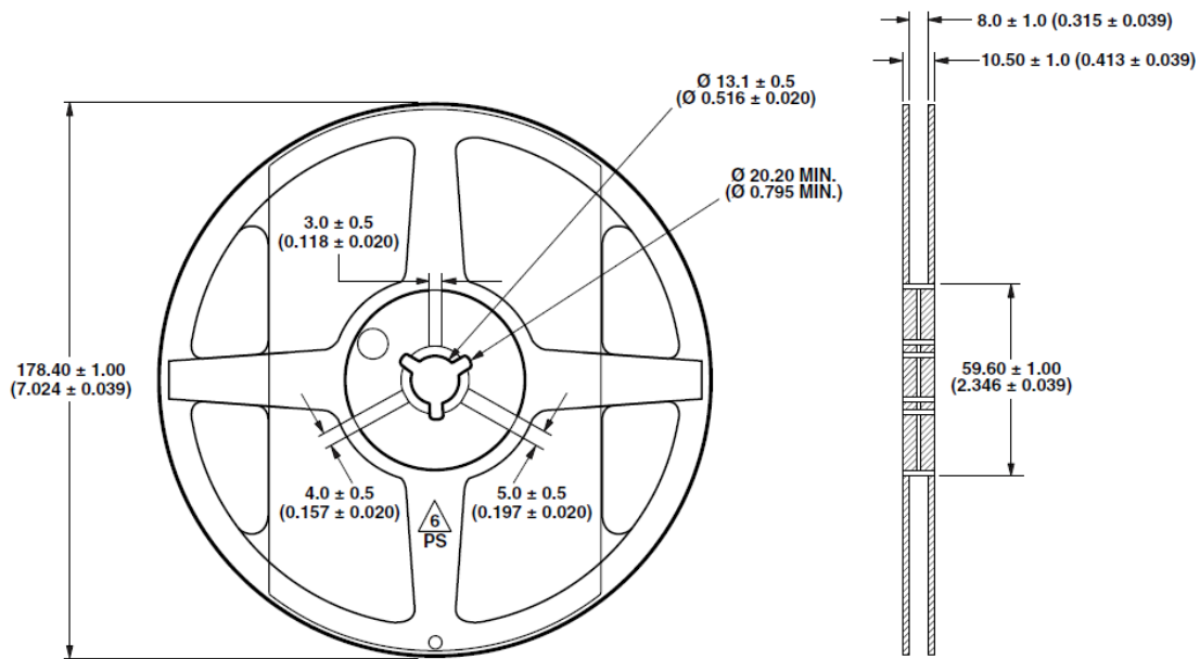
Figure 10. Reel orientation
