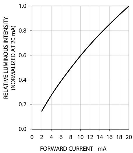
Figure 2. Luminous Intensity vs Forward Current
