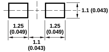
HSMX-H670 SERIES
