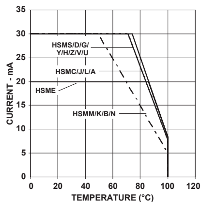
Figure 4. Maximum forward current vs. ambient temperature. Derated based on T_J\text{MAX} = 110^\circ\text{C} , R\theta_{JA} = 500^\circ\text{C/W} .
