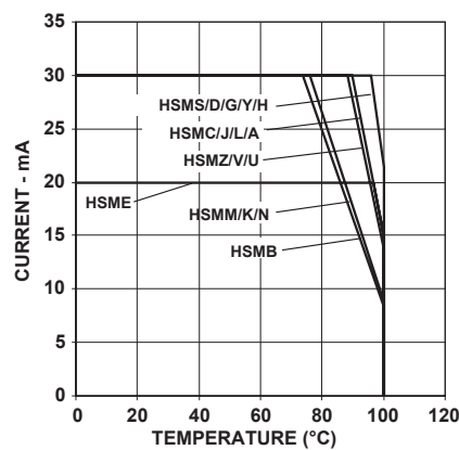
Figure 4b. Maximum Forward Current Vs. Solder Point Temperature. Derated based on T_J\text{MAX} = 110^\circ\text{C} , R\theta_{JP} = 180^\circ\text{C/W} or 280^\circ\text{C/W} .
