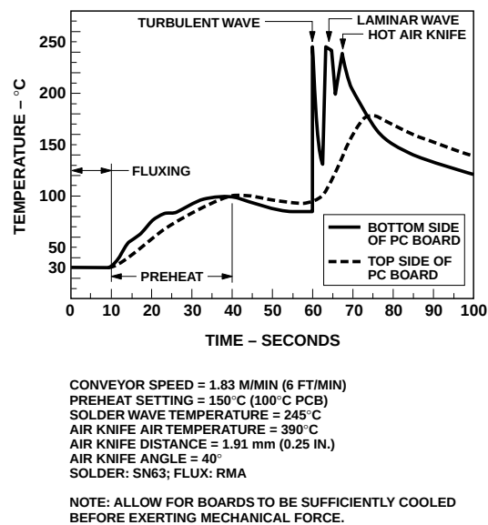
Figure 9. Recommended wave soldering profile.
