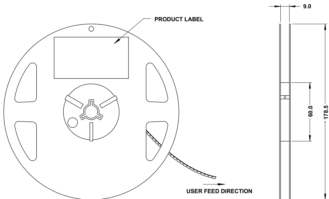
Figure 9: Reel Dimensions
