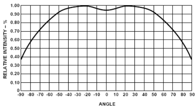
Figure 5: Radiation Pattern
