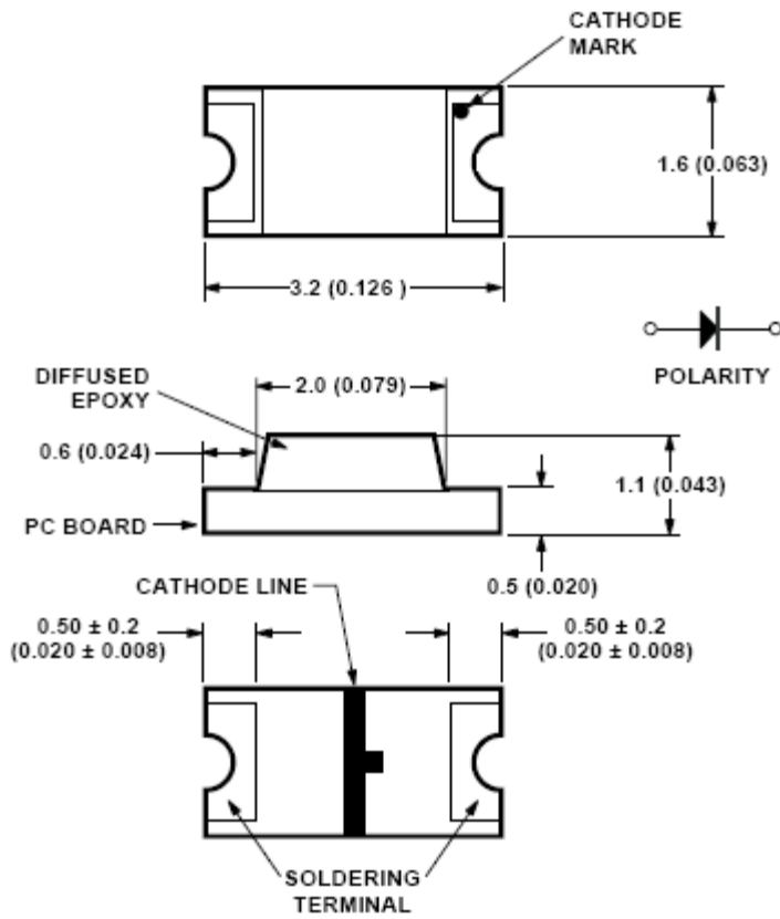
Figure 1: Package Dimensions
