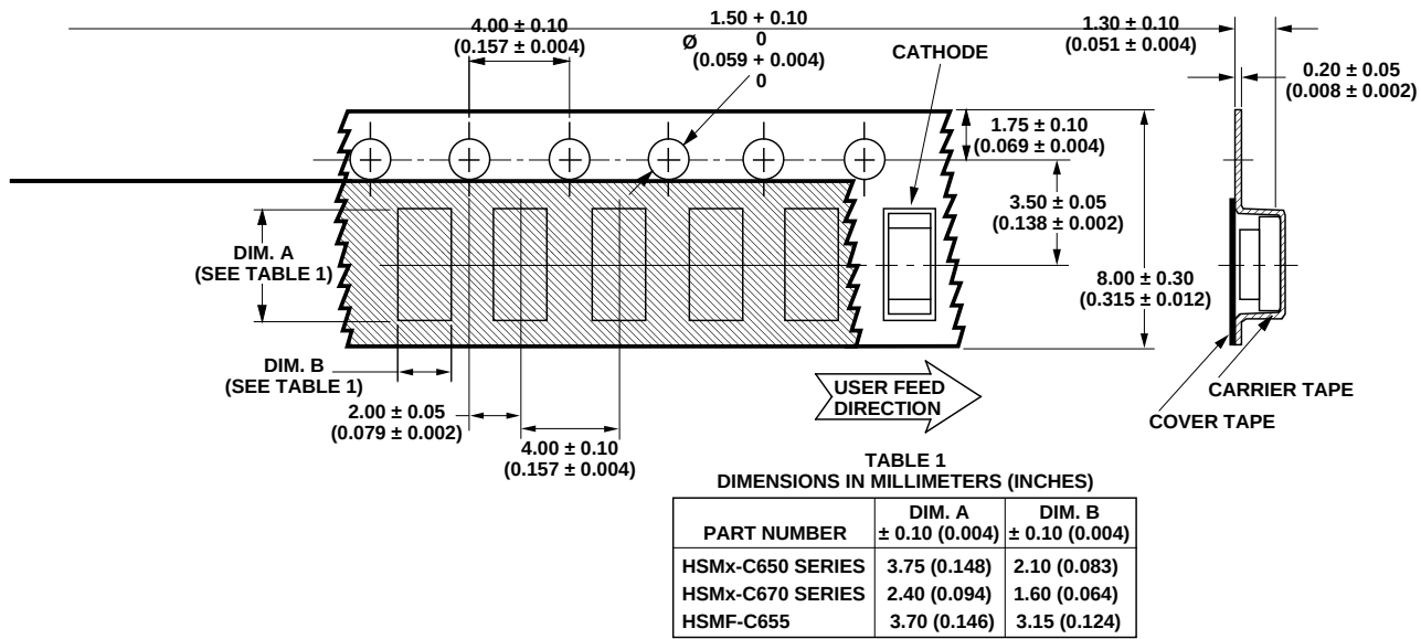
Figure 10. Tape Dimensions.
