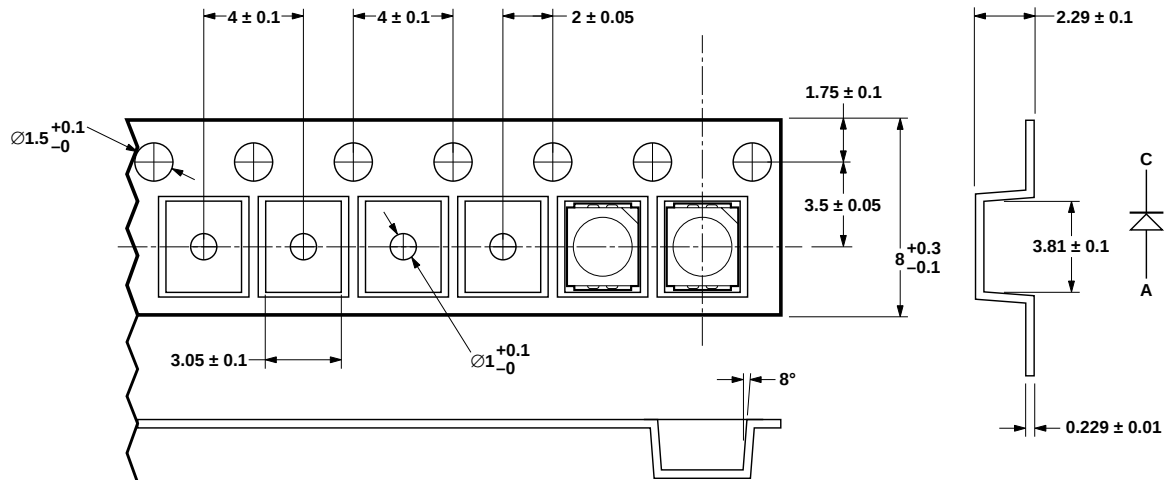
Figure 12. Tape dimensions.
