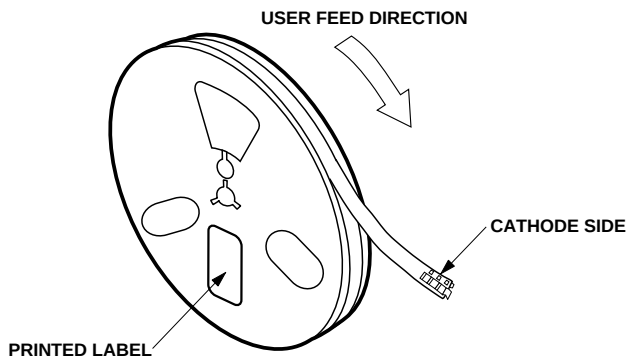
Figure 14. Reeling orientation.
