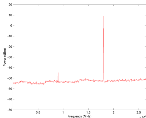
Figure 14b: 18GHz Broad Band Spectrum
