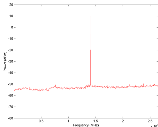
Figure 12b: 14GHz Broad Band Spectrum
