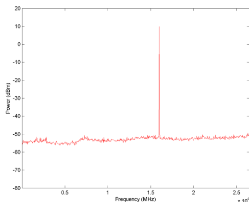
Figure 13b: 16GHz Broad Band Spectrum
