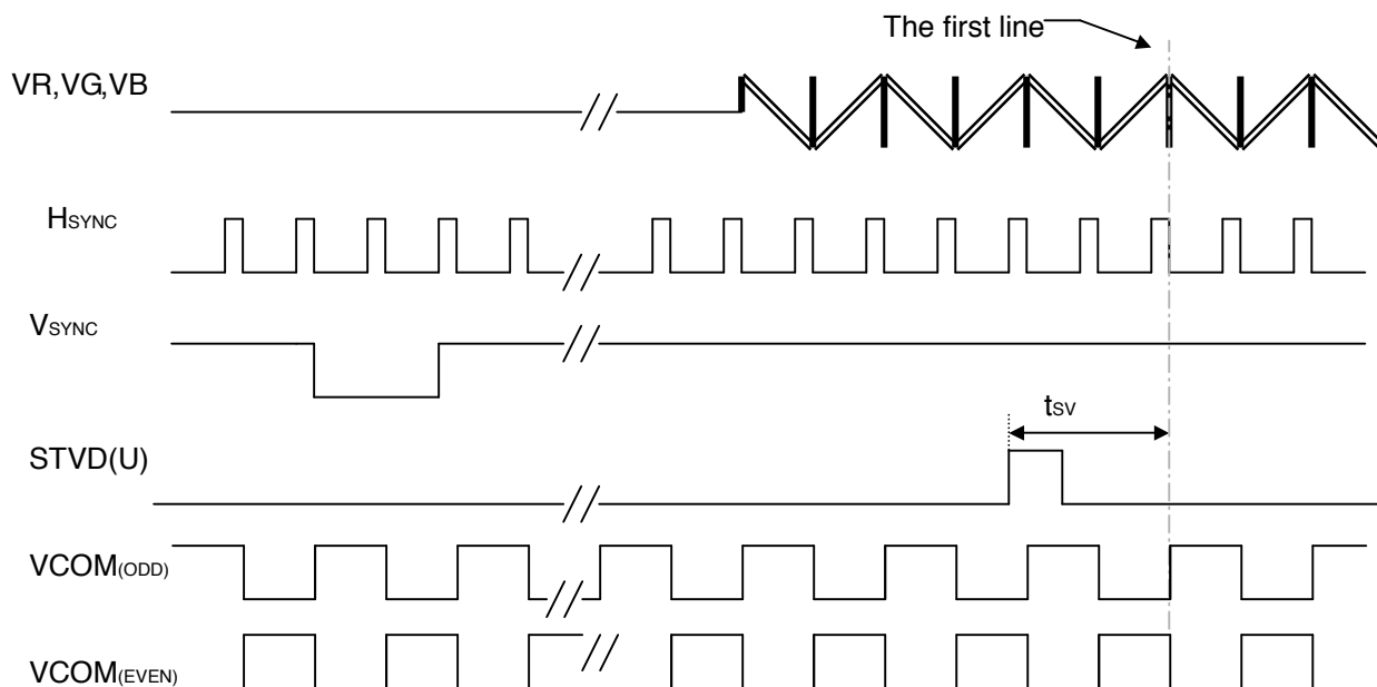
Vertical timing
