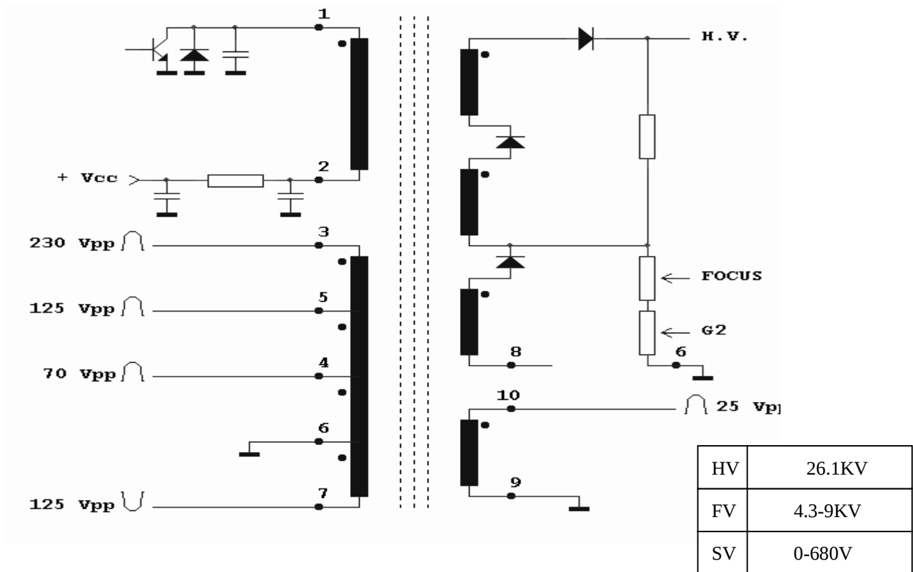
HR8342
