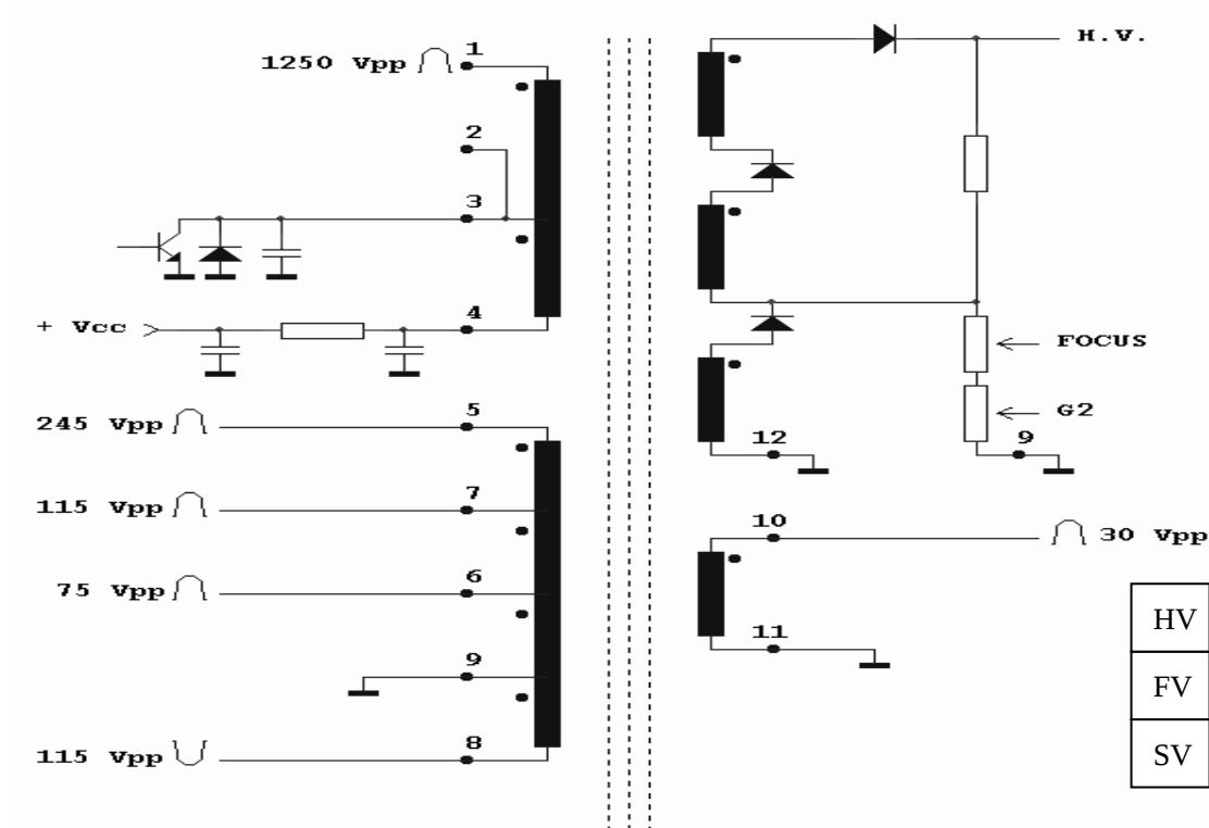
HR8316
