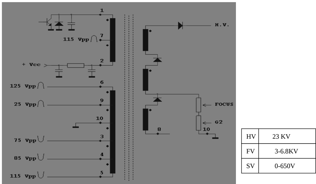
HR8342
