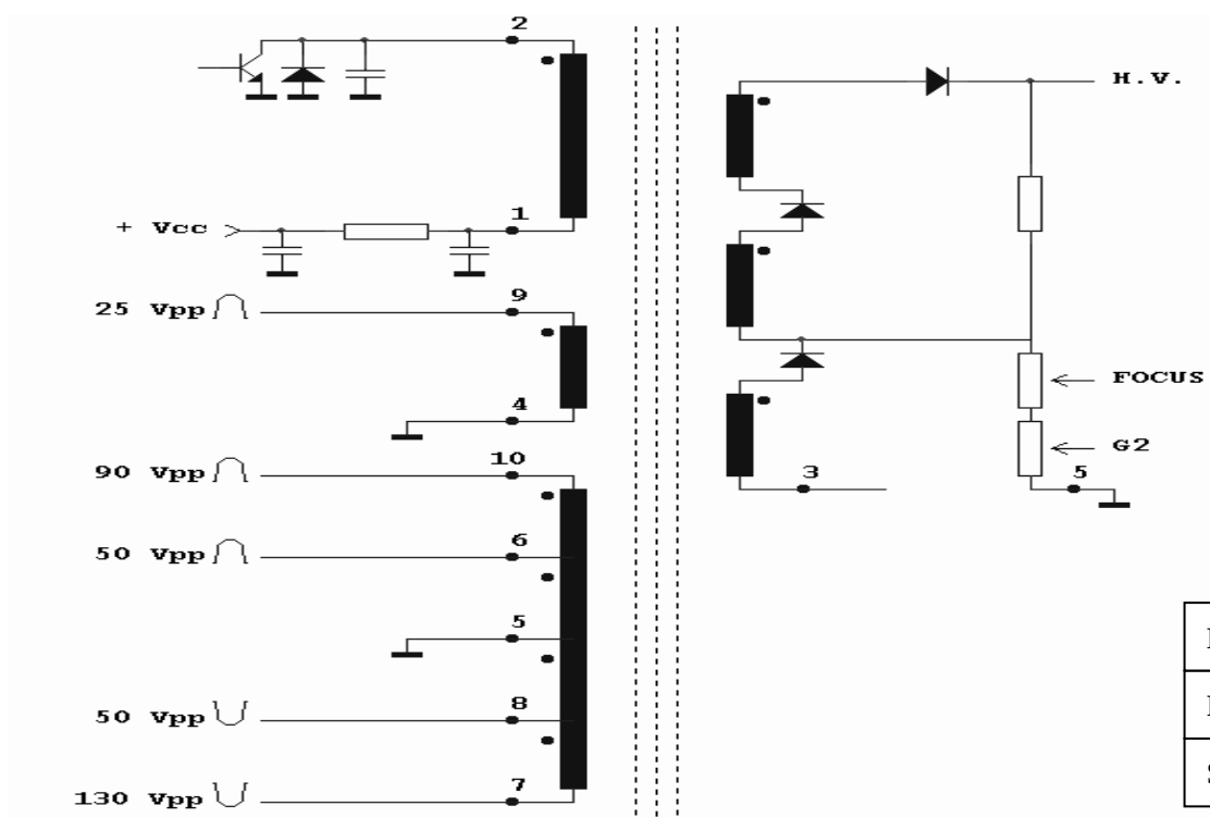
HR8316
