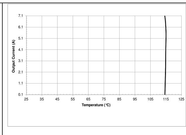
HQA2W085W120V maximum output current vs. baseplate temperature at nominal line
