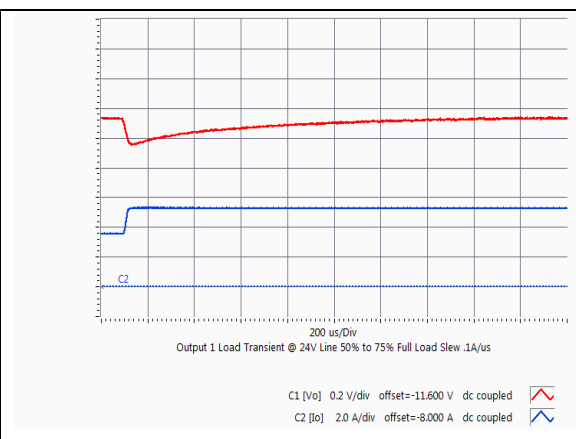
HQA2W085W280V Typical transient response. Output voltage response to load step from 50% to 75% of full load with output current slew rate of 0.1A/uS.
