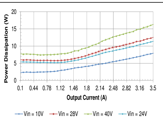
HQA2W085W240V Typical Power Dissipation vs. Input Voltage at Ta=25 degrees
