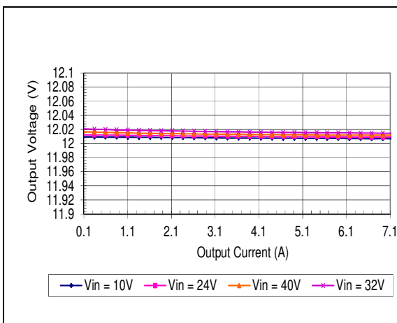
HQA2W085W120V Typical Load Regulation Characteristics at Ta=25 degrees.
