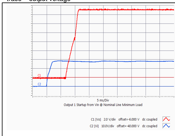
HQA2W085W150V Typical startup characteristic from input voltage application at light load. Red trace - output voltage, Blue trace -input voltage
