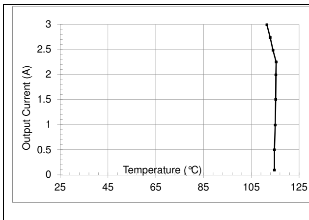
HQA2W085W280V maximum output current vs. baseplate temperature
