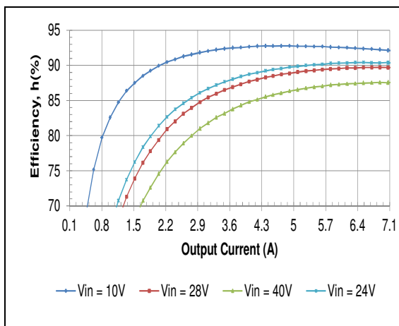
HQA2W085W120V Typical Efficiency vs. Input Voltage at Ta=25 degrees.
