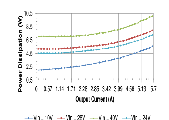
HQA2W085W150V Typical Power Dissipation vs. Input Voltage at Ta=25 degrees
