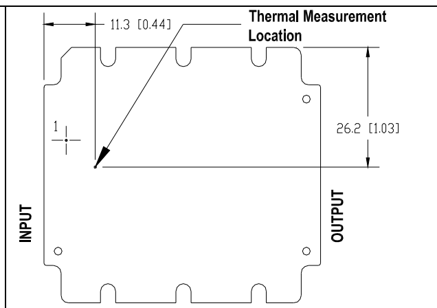
HQA2W085W280V-007 thermal measurement location – top view
