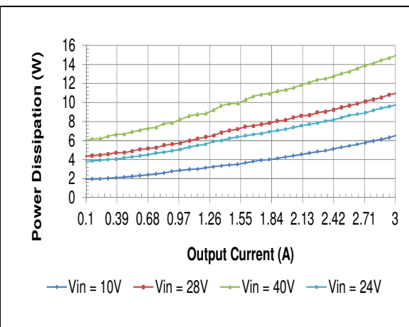
HQA2W085W280V Typical Power Dissipation vs. Input Voltage at Ta=25 degrees
