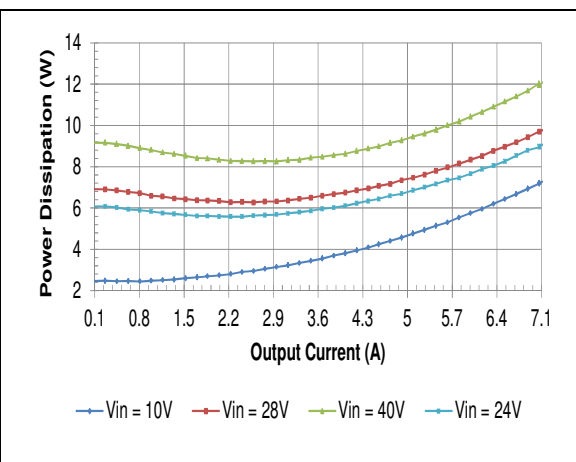
HQA2W085W120V Typical Power Dissipation vs. Input Voltage at Ta=25 degrees
