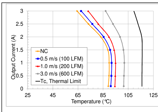
HQA2W085W280V maximum output current vs. ambient temperature at 28V input for airflow rates natural convection (60lfm) to 600lfm with airflow from pin 3 to pin 1
