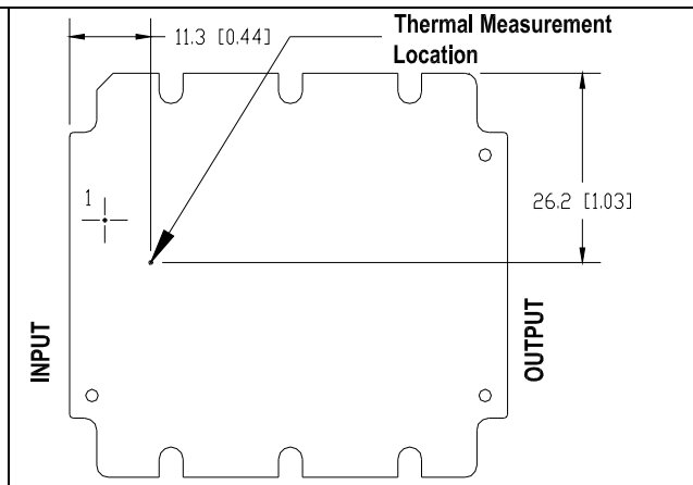
HQA2W085W150V thermal measurement location – top view
