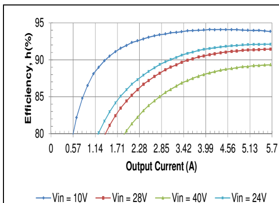
HQA2W085W150V Typical Efficiency vs. Input Voltage at Ta=25 degrees.
