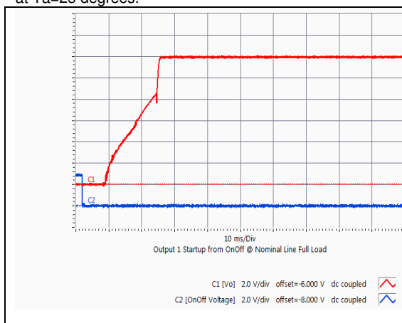
HQA2W085W120V Typical startup characteristic from on/off at full load. Lower trace - on/off signal, upper trace – output voltage
