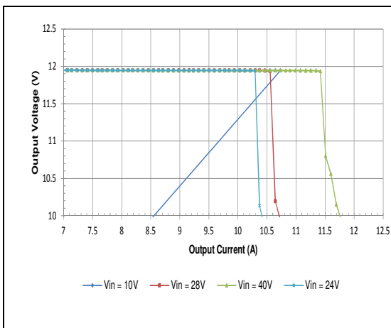
HQA2W085W120V Typical Output Current Limit Characteristics vs. Input Voltage at Ta=25 degrees.
