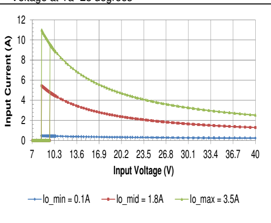
HQA2W085W240V Typical Input Current vs. Input Voltage Characteristics
