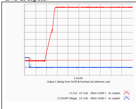
HQA2W085W150V Typical startup characteristic from on/off at light load. Lower trace - on/off signal, upper trace - output voltage
