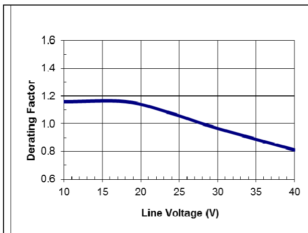
HQA2W085W120V typical temperature derating versus input voltage output with 2m/s (400 lfm) airflow from pin 3 to pin 1.
