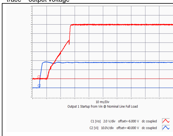
HQA2W085W120V Typical startup characteristic from input voltage application at full load. Red trace - output voltage, Blue trace –input voltage
