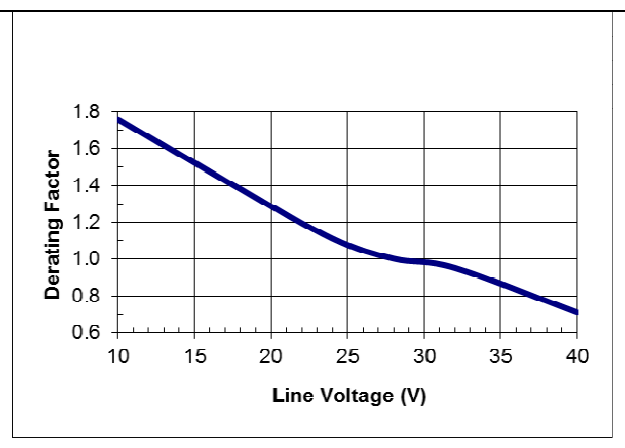
HQA2W085W280V typical temperature derating versus input voltage output with 2m/s (400 lfm) airflow from pin 3 to pin 1.
