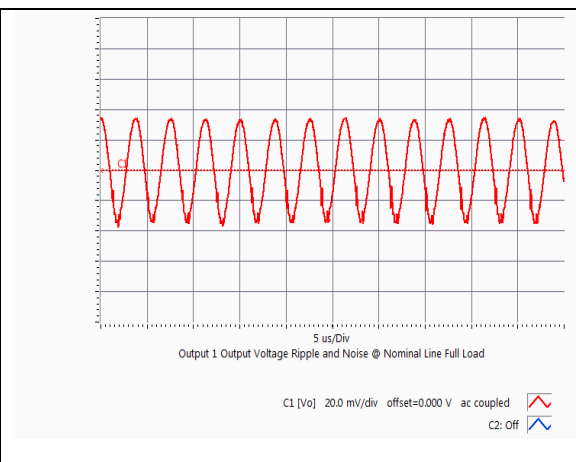
HQA2W085W120V Typical Output Ripple at nominal Input voltage and full load at Ta=25 degree
