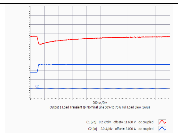
HQA2W085W120V Typical output voltage response to load step from 50% to 75% of full load with output current slew rate of 0.1A/uS and Cext = 500uF
