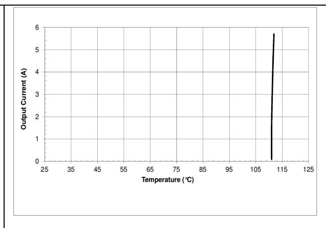
HQA2W085W150V maximum output current vs. baseplate temperature at nominal line
