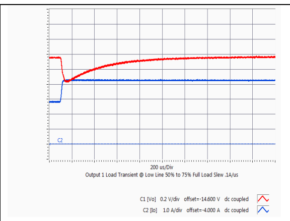
HQA2W085W150V Typical output voltage response to load step from 50% to 75% of full load with output current slew rate of 0.1A/uS and Cext = 10uF
