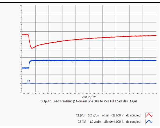
HQA2W085W240V Typical transient response. Output voltage response to load step from 50% to 75% of full load with output current slew rate of 0.1A/uS.
