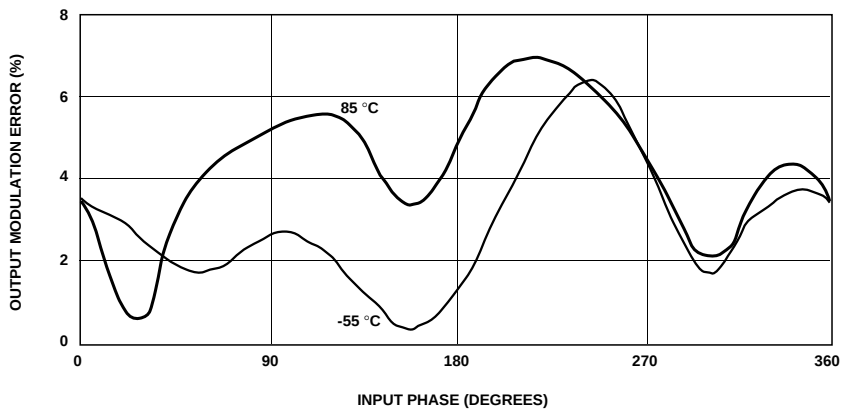
Figure 14. Modulation Error vs. Input Phase at 900 MHz, V_{CC} = 5\text{ V} , \sqrt{(V_{I_{mod}} - 2.5)^2 + (V_{Q_{mod}} - 2.5)^2} = 1.25\text{ V} , LO = -12 dBm. Percent Modulation Error is Calculated from the Values of Amplitude and Phase Error.
