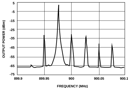
Figure 15. Single Sideband Output Spectrum. LO = -12 dBm at 900 MHz. The Test Setup is Shown in Figure 17.
