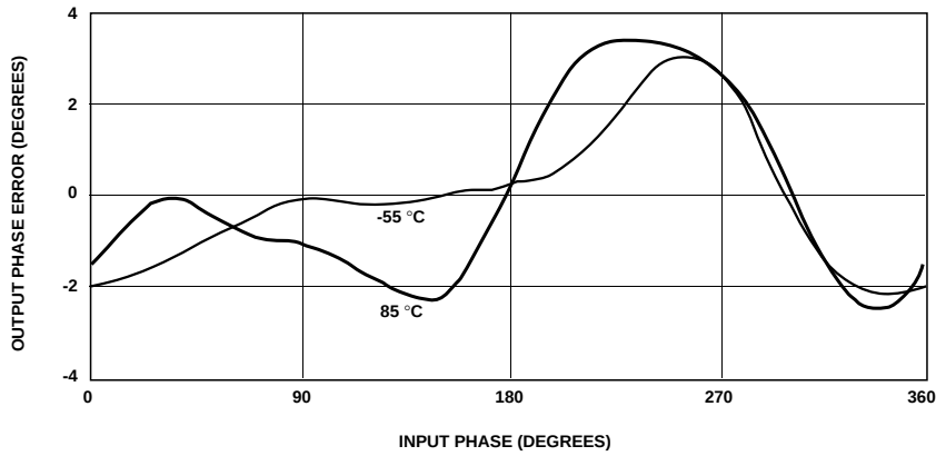
Figure 13. HPMX-2003 Output Phase Error vs. Input Phase at 900 MHz, V_{CC} = 5\text{ V} , \sqrt{(V_{I_{mod}} - 2.5)^2 + (V_{Q_{mod}} - 2.5)^2} = 1.25\text{ V} , LO = -12 dBm. 25°C Curve Deleted for Clarity.
