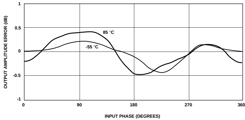
Figure 12. HPMX-2003 Amplitude Error vs. Input Phase at 900 MHz, V_{CC} = 5\text{ V} , \sqrt{(V_{I_{mod}} - 2.5)^2 + (V_{Q_{mod}} - 2.5)^2} = 1.25\text{ V} , LO = -12 dBm. 25°C Curve Deleted for Clarity.
