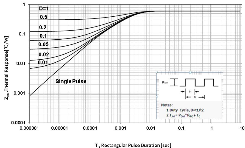
Figure.5 Maximum Effective Thermal Impedance , Junction to Case
