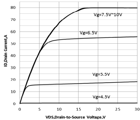
Figure.4 Typical Output Characteristics
