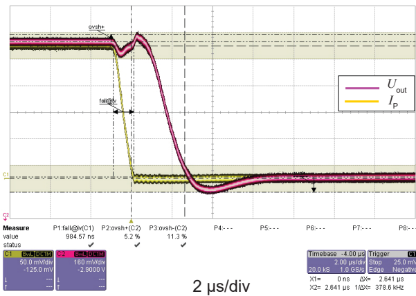
Figure 13: Step response
