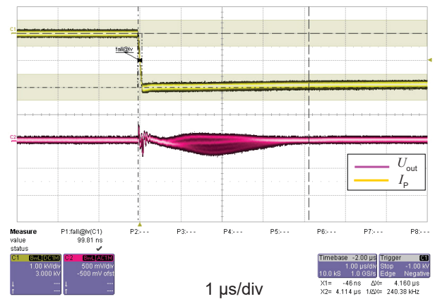
Figure 14: dv/dt
