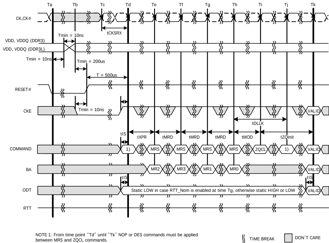
Figure 0 - VDD/VDDQ Voltage Switch Between DDR3L and DDR3
