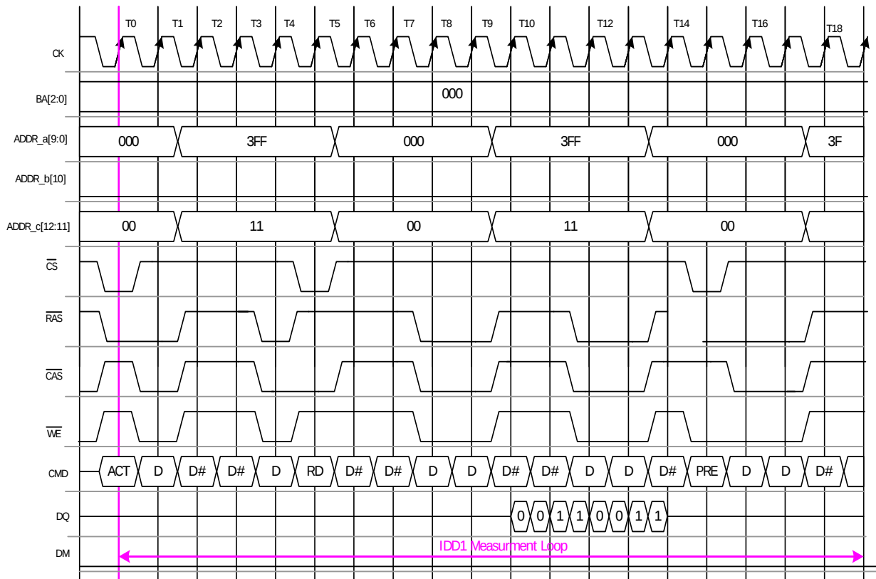
< Figure 1. IDD1 Example > (DDR3-800-555, 512Mb x8): Data DQ is shown but the output buffer should be switched off (per MR1 Bit A12 = "1") to achieve I_{out} = 0\text{mA} . Address inputs are split into 3 parts.
