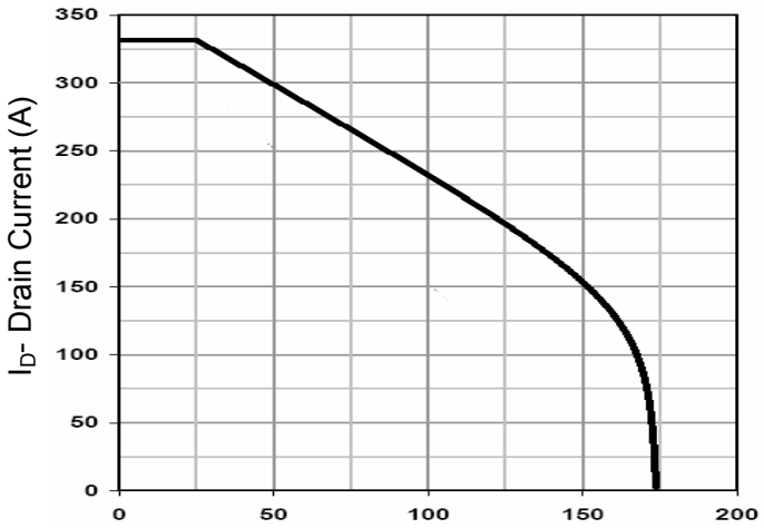
T_J -Junction Temperature ( ^{\circ}\text{C} ) Figure 10 Current De-rating
