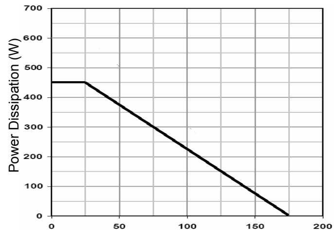
T_J -Junction Temperature ( ^{\circ}\text{C} ) Figure 9 Power De-rating
