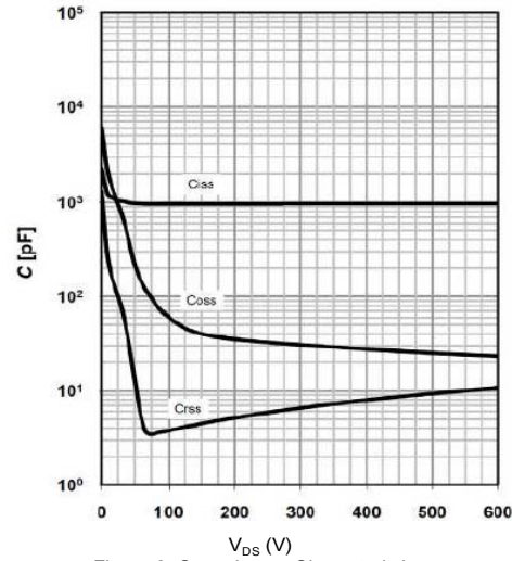
Figure 9: Capacitance Characteristics
