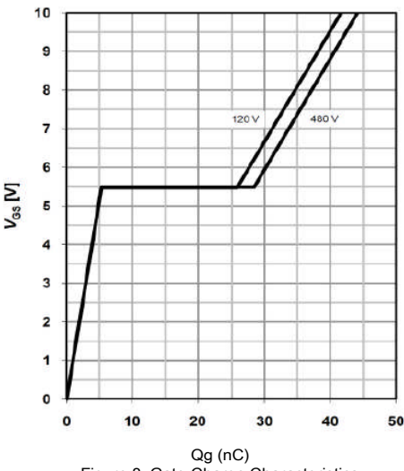
Figure 8: Gate-Charge Characteristics
