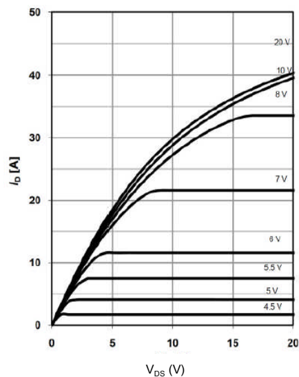
Figure 1: On-Region Characteristics@25°C
