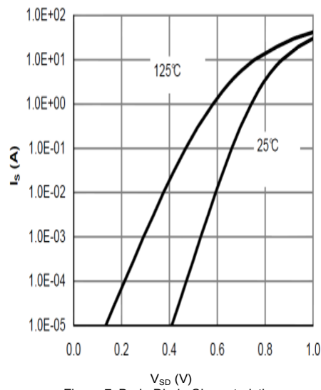
Figure 7: Body-Diode Characteristics
