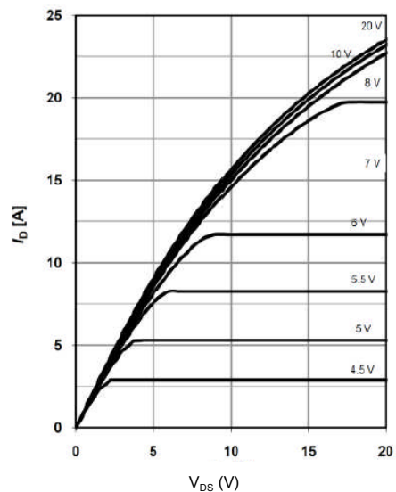
Figure 2: On-Region Characteristics@125°C
