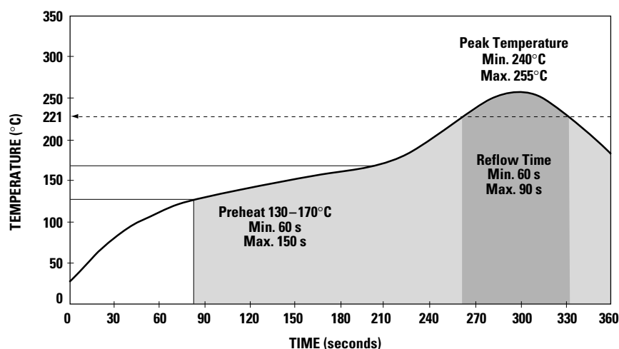
Figure 14. Surface Mount Assembly Temperature Profile.
