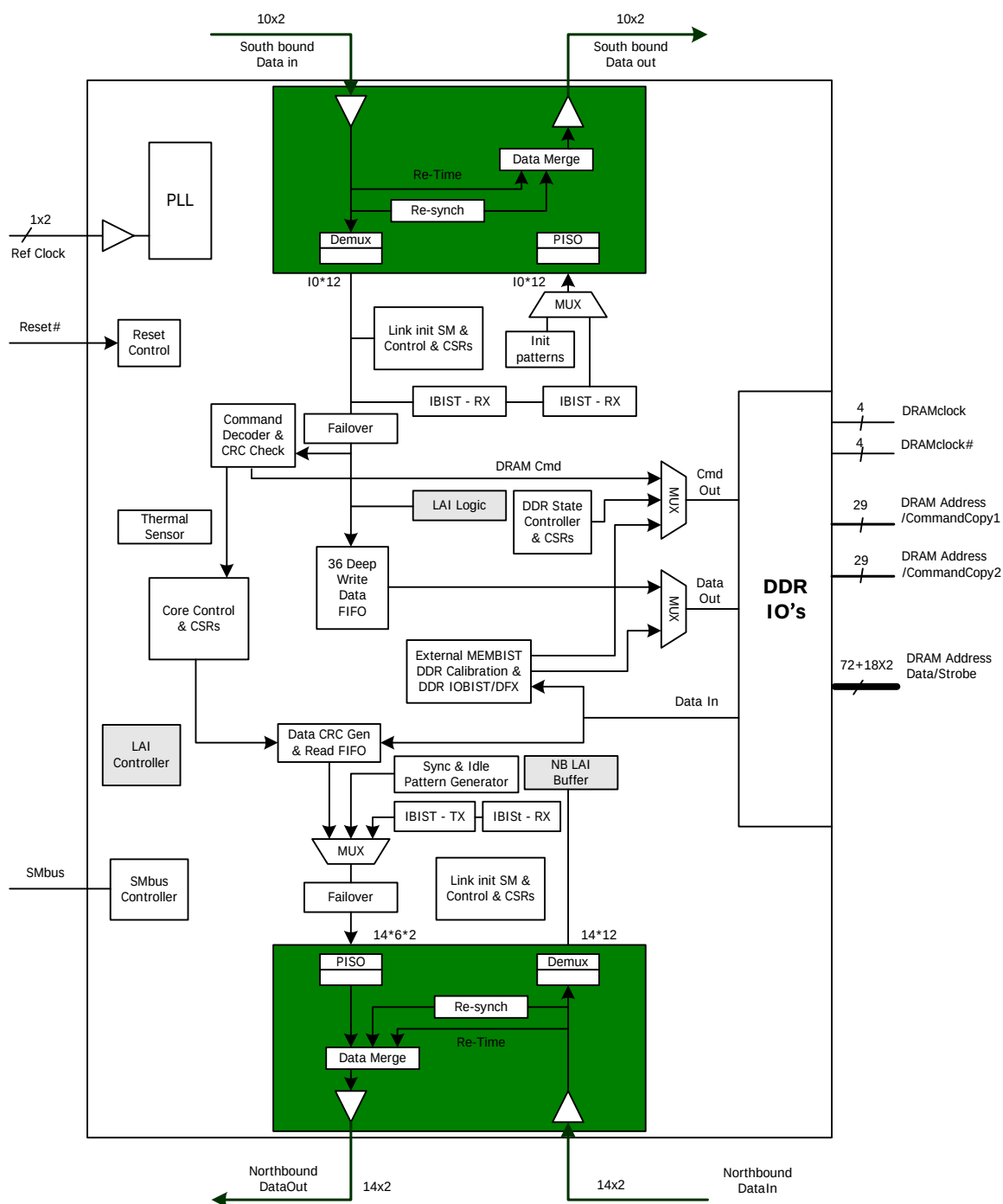
Advanced Memory Buffer Block Diagram
