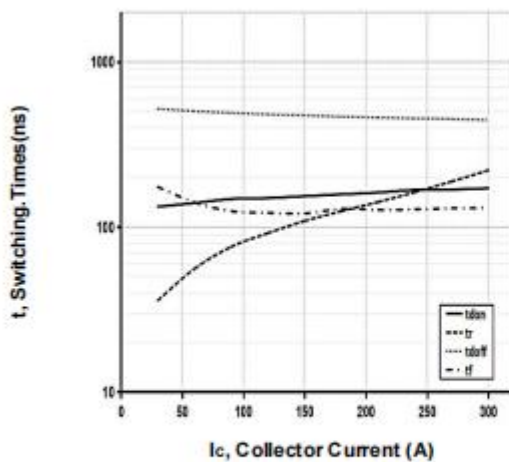
Figure 5. Typical switching times vs. collector current (Ind. load, T_j = 175^\circ\text{C} , V_{CE} = 400\text{V} , V_{GE} = 15/0\text{V} , R_G = 10\Omega )
