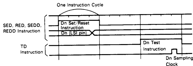
Figure 16 Timing Chart of Discrete I/O
