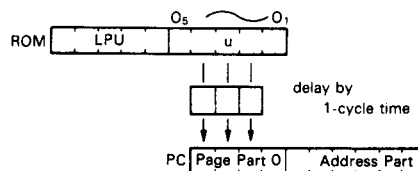
Figure 8 LPU Operation
