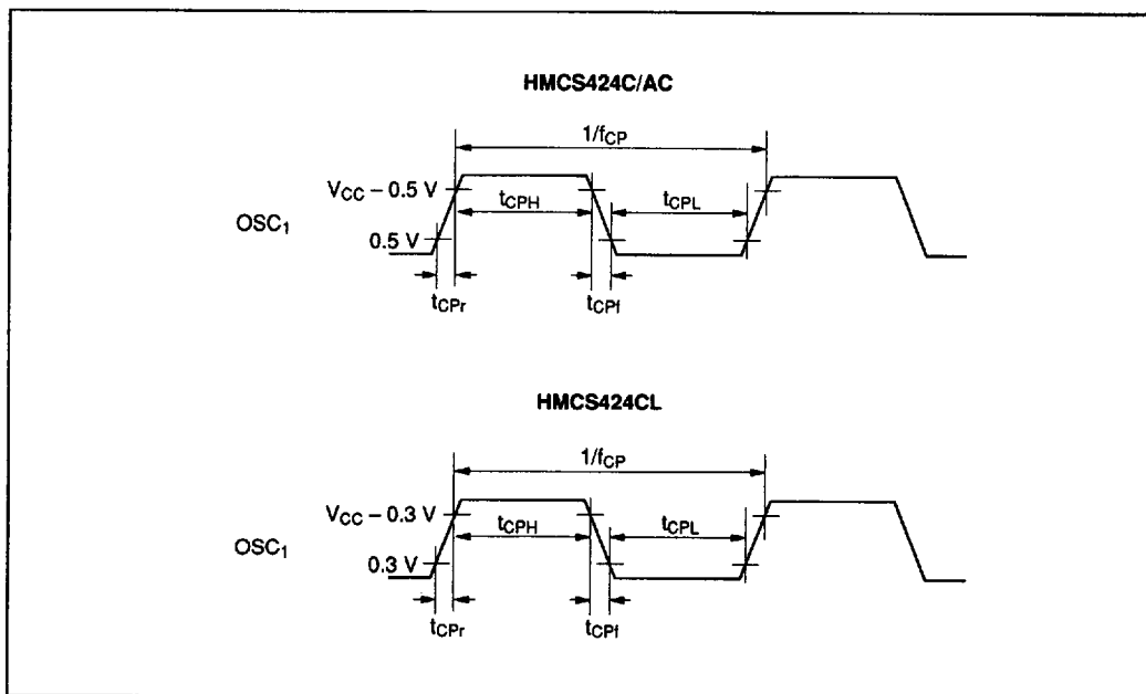
Figure 33 Oscillator Timing
