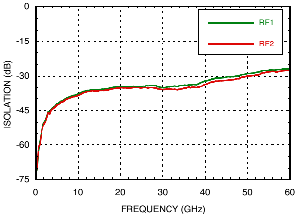
Isolation @-5V
