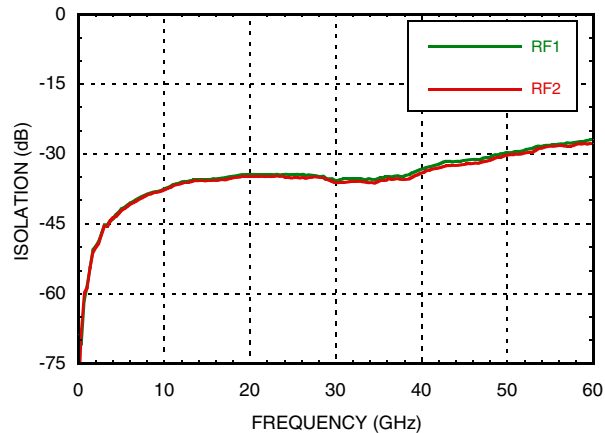
Isolation @-3V
