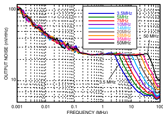
Figure 4. Filter Output Noise
