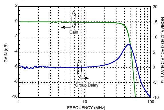
Figure 14. 50 MHz Filter Magnitude and Group Delay
