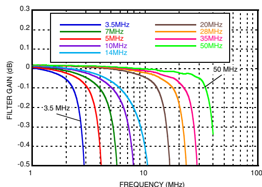
Figure 3. Filter Passband Gain Response
