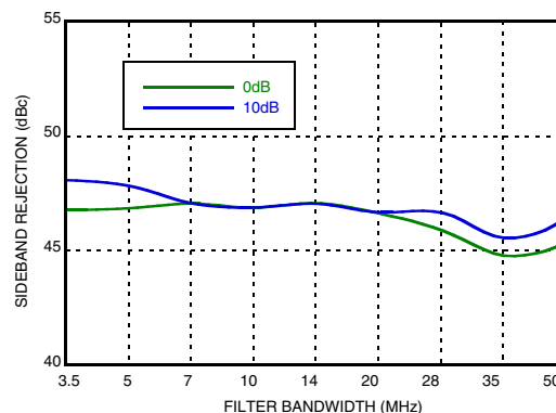
Figure 6. Filter Side Band Rejection vs Bandwidth
