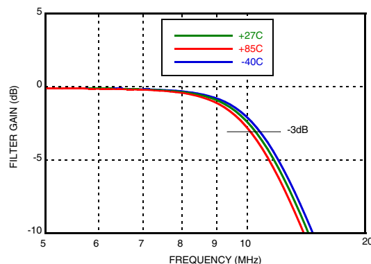
Figure 5. Filter 3 dB Cutoff vs Temperature, 10 MHz Bandwidth
