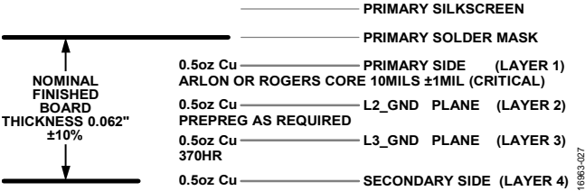
Figure 27. 4-Layer Stackup
