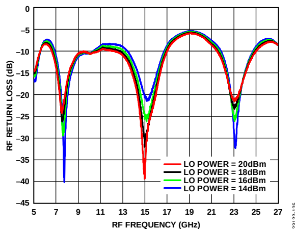
Figure 125. RF Return Loss vs. RF Frequency at Various LO Drives, LO Frequency = 16 GHz
