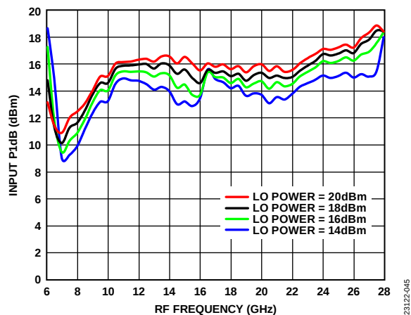
Figure 45. Input P1dB vs. RF Frequency at Various LO Drives, T_A = 25^\circ\text{C}
