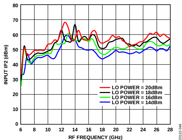
Figure 46. Input IP2 vs. RF Frequency at Various LO Drives, T_A = 25^\circ\text{C}
