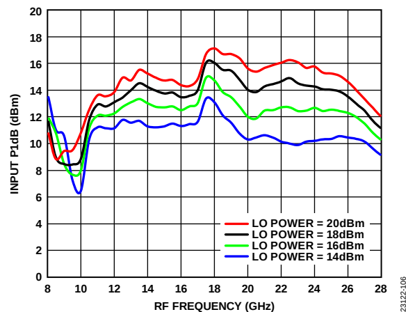
Figure 106. Input P1dB vs. RF Frequency at Various LO Drives, T_A = 25^\circ\text{C}
