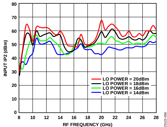
Figure 56. Input IP2 vs. RF Frequency at Various LO Drives, T_A = 25^\circ\text{C}
