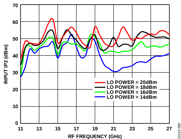
Figure 66. Input IP2 vs. RF Frequency at Various LO Drives, T_A = 25^\circ\text{C}
