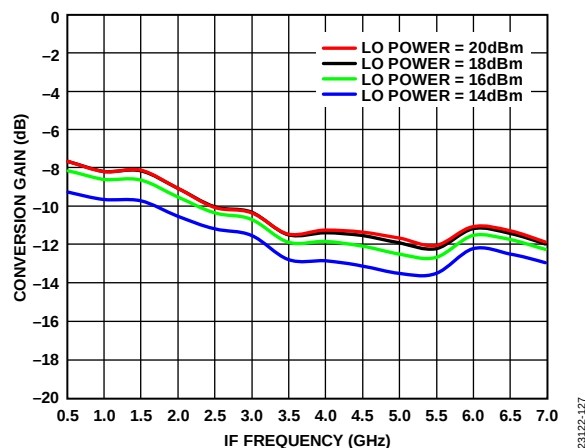
Figure 130. Conversion Gain vs. IF Frequency at Various LO Drives, LO Frequency = 16 GHz, T_A = 25^\circ\text{C}
