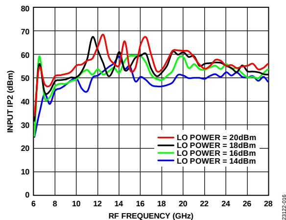
Figure 16. Input IP2 vs. RF Frequency at Various LO Drives, T_A = 25^\circ\text{C}
