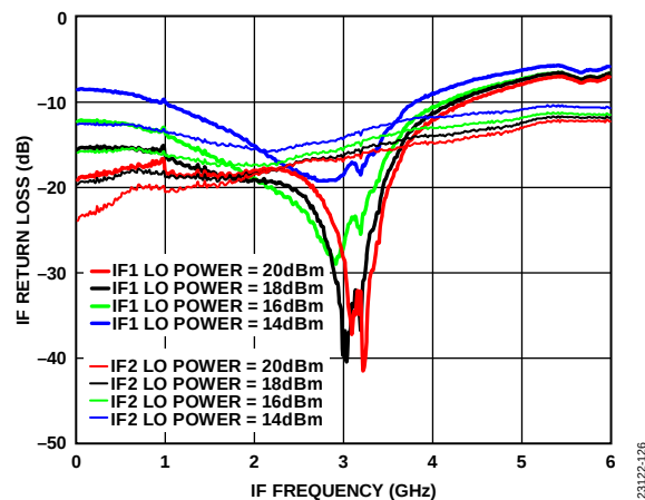
Figure 126. IF Return Loss vs. IF Frequency at Various IFx LO Drives, LO Frequency = 16 GHz
