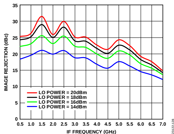
Figure 131. Image Rejection vs. IF Frequency at Various LO Drives, LO Frequency = 16 GHz, T_A = 25^\circ\text{C}
