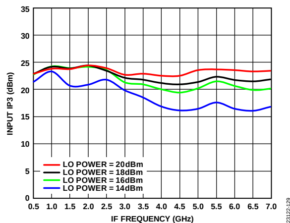
Figure 132. Input IP3 vs. IF Frequency at Various LO Drives, LO Frequency = 16 GHz, T_A = 25^\circ\text{C}
