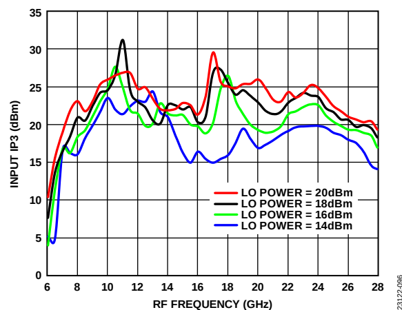
Figure 96. Input IP3 vs. RF Frequency at Various LO Drives, T_A = 25^\circ\text{C}
