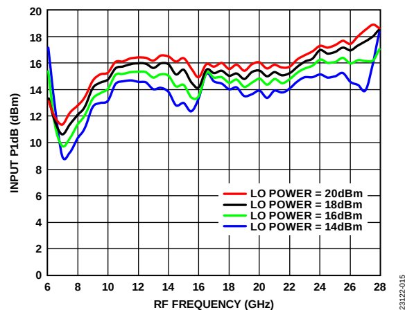
Figure 15. Input P1dB vs. RF Frequency at Various LO Drives, T_A = 25^\circ\text{C}
