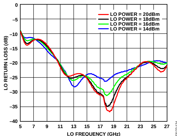
Figure 124. LO Return Loss vs. LO Frequency at Various LO Drives at T_A = 25^\circ\text{C}
