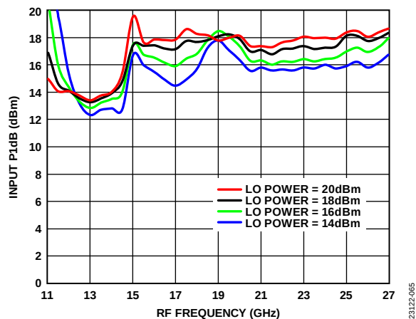
Figure 65. Input P1dB vs. RF Frequency at Various LO Drives, T_A = 25^\circ\text{C}
