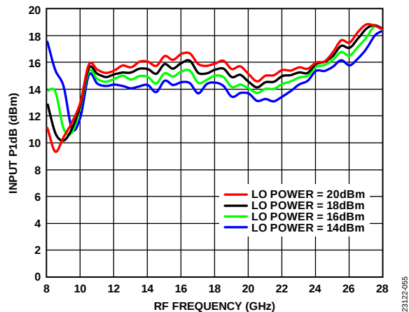
Figure 55. Input P1dB vs. RF Frequency at Various LO Drives, T_A = 25^\circ\text{C}
