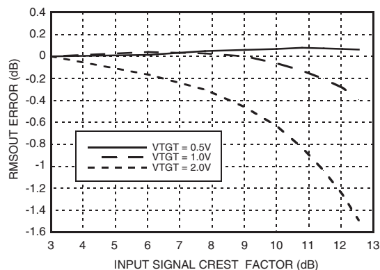
RMS Error vs. Crest Factor Over VTGT [2]
