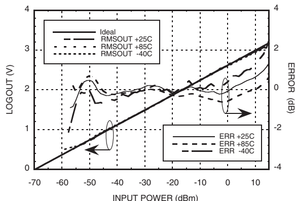
RMSOUT & Error vs. Pin @ 100 MHz [1]
