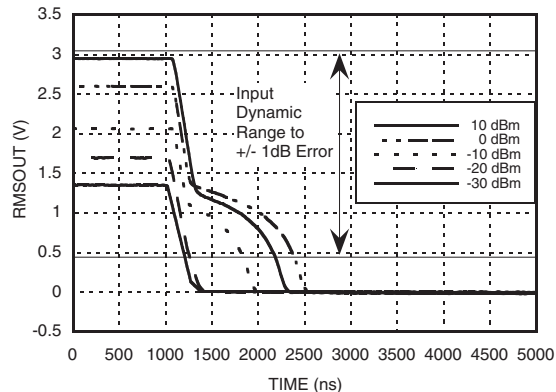
Output Response
