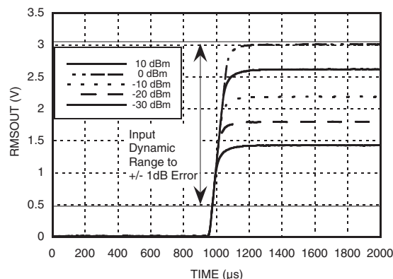
Output Response
