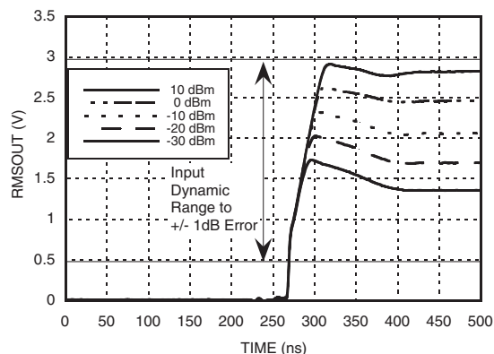
Output Response
