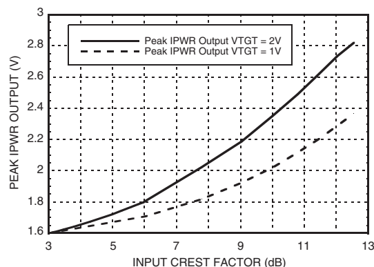
Peak IPWR vs Input Crest Factor [5]
