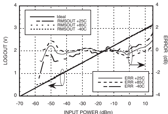
RMSOUT & Error vs. Pin @ 900 MHz [1]
