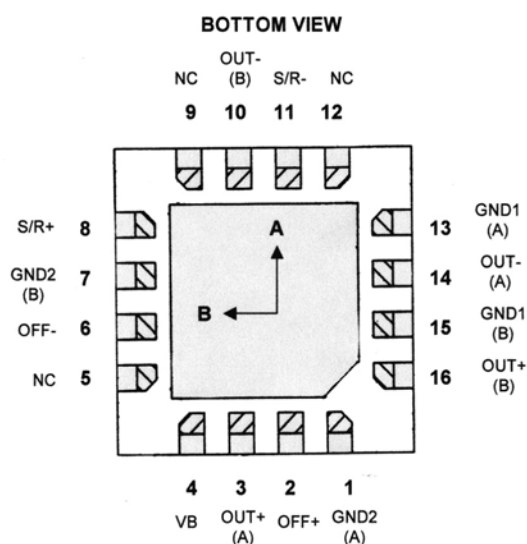
HMC1052 Pinout
