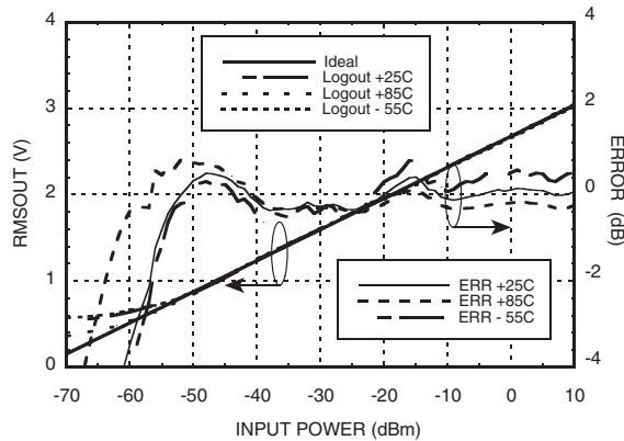
www.datasheet4u.com RMSOUT & Error vs. Pin @ 10 MHz [1]
