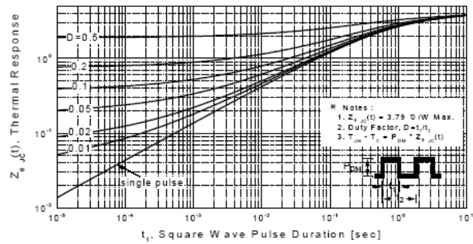
Figure 11-2. Transient Thermal Response Curve for HM9N50I
