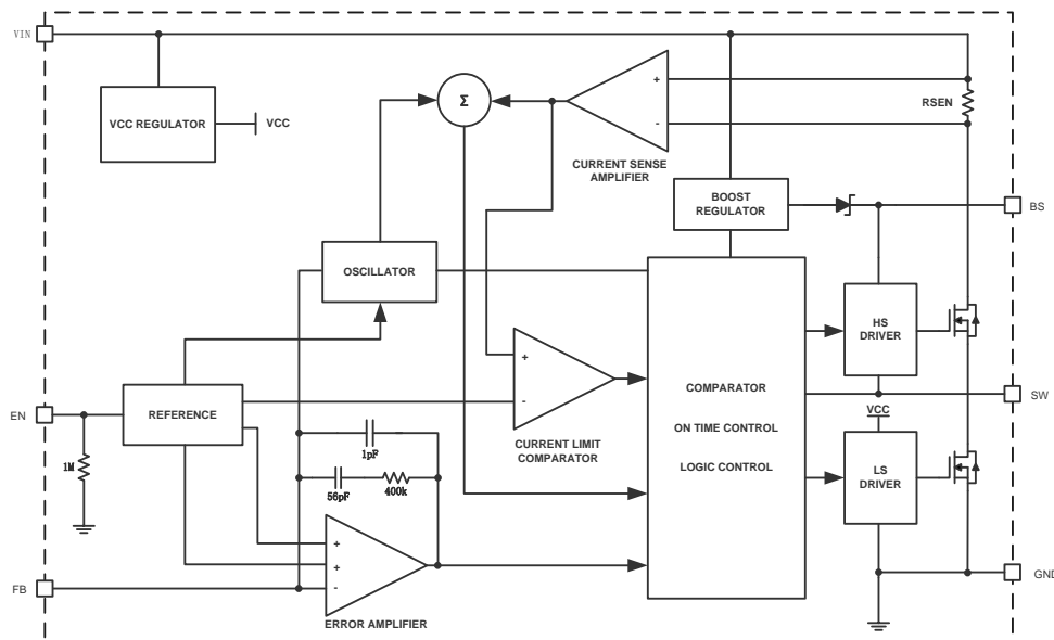
Figure 2. HM8114 Block Diagram
