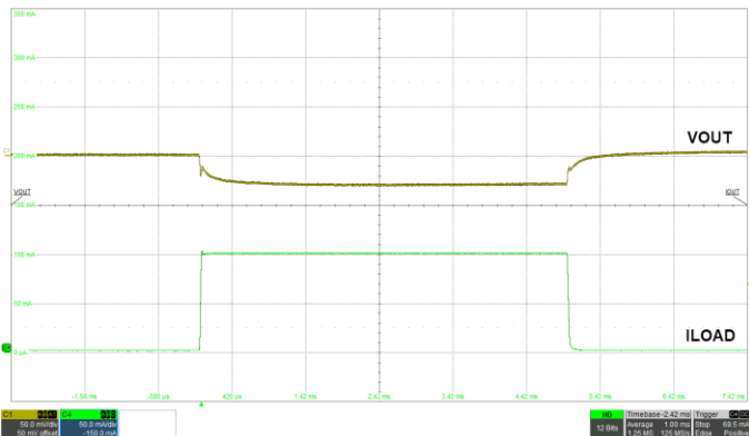
Fig 10. Load Transient(1mA to 100mA)
