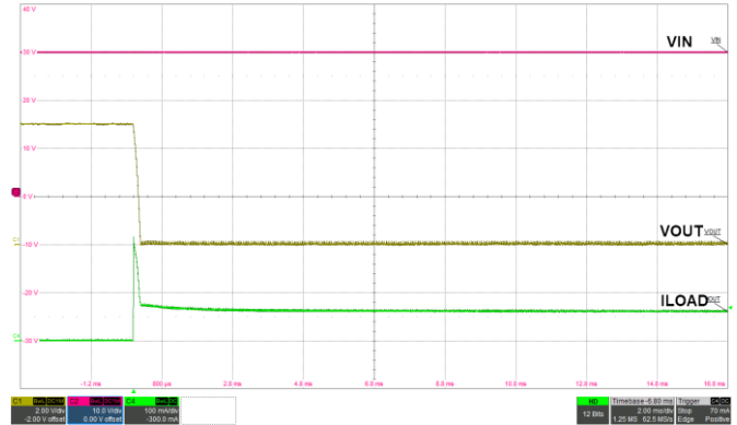
Fig 8. VOUT Short to GND
