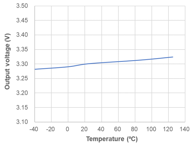
Fig 4. V_{OUT}=3.3V vs Temp
