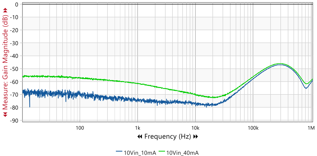
Fig 10. PSRR vs Frequency ( V_{IN} = 10V , V_{OUT} = 5V )
