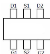
SOT-23-6L top view
