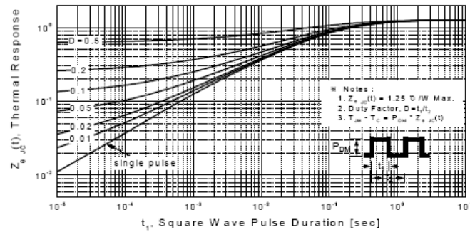
Figure 11-1. Transient Thermal Response Curve for HM5N65
