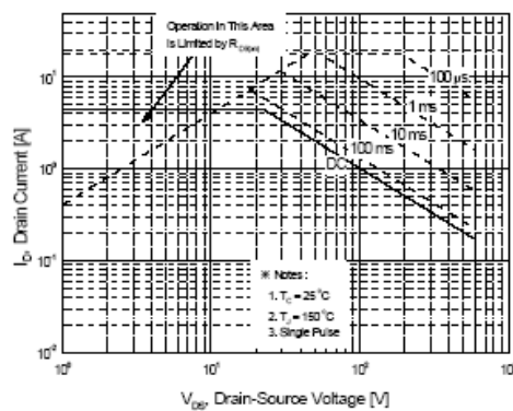
Figure 9-1. Maximum Safe Operating Area for HM5N65
