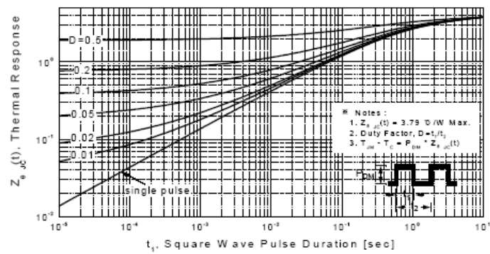
Figure 11-2. Transient Thermal Response Curve for HM5N65F
