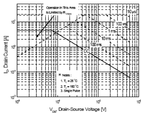
Figure 9-2. Maximum Safe Operating Area for HM5N65F
