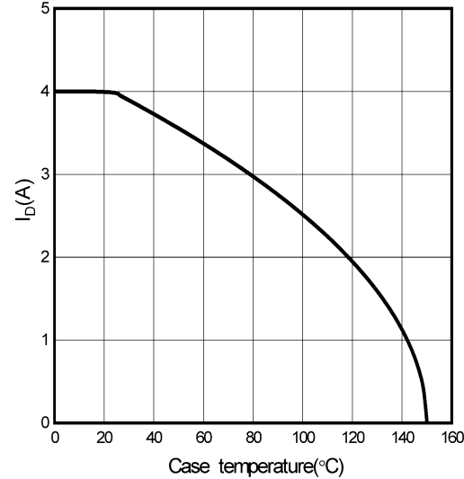
Figure 11.Drain Current Derating
